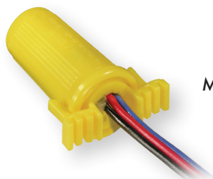
LV9000 Min #24/Max #18
